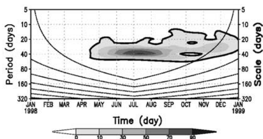
Figure 2. The local wavelet power spectrum of the normalized and 20–120-day filtered convective index over the SCS in 1998 using the Morlet wavelet. The left axis is the Fourier period (in day) corresponding to the wavelet scale on the right axis. The bottom axis is time (day). The thick contour encloses regions of greater than 99% confidence for a red-noise process with a lag-1 coefficient of 0.98. The dotted line covered regions on either end indicate the “cone of influence,” where edge effects become important.
