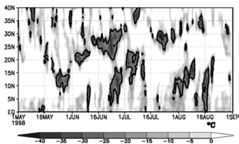
Figure 1. Time-latitude cross-section of GMS IR temperature between 110\text{--}120^\circ\text{E} , the temperature less than -25^\circ\text{C} is enclosed by the thick lines.
