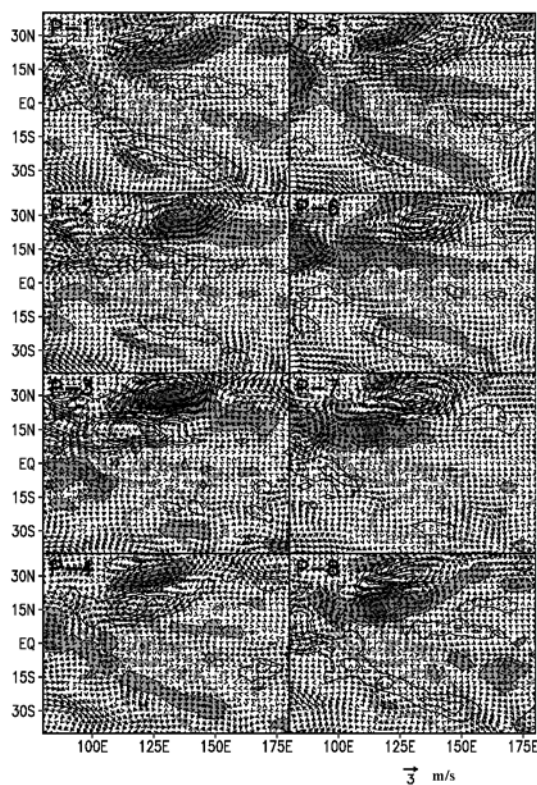
Figure 5. Regression maps of OLR based on the first two EOFs and 30–60-day filtered wind vector at low-level of 850 hPa for every 45^\circ of phase \alpha of 30–60 day ISO. The OLR contour interval is 5 \text{ W m}^{-2} ; the first positive contour is at 5 \text{ W m}^{-2} ; negative contours are dotted; shading is shown by the legend. The category of phase number of P-1 to 8 is also shown in the maps.
