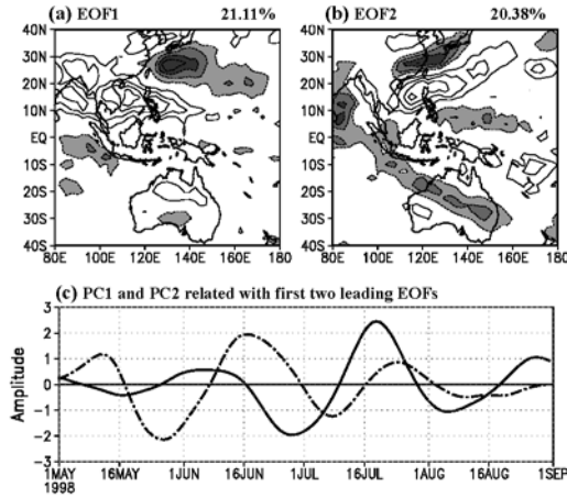
Figure 4. Empirical orthogonal function (EOF) analysis of 20–120-day filtered OLR. (a) EOF1, (b) EOF2; contour interval is 5 \text{ W m}^{-2} ; the zero contour is omitted; shading is shown by the legend. (c) PC1 (solid line) and PC2 (dashed line) from 1 May to 31 August 1998.
