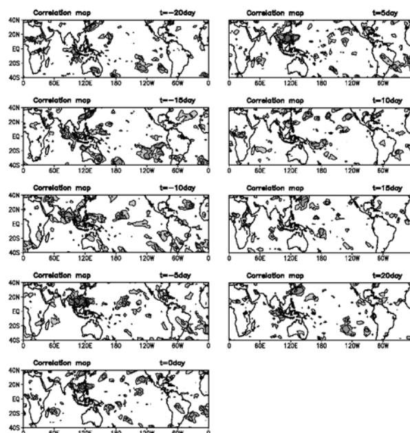
Figure 3. Lagged correlation maps of positive coefficients, greater than 99% confidence between the 30–60-day SCS convective index and 20–120-day filtered OLR in the summer of 1998 for the day -20 to day 20 with 5 days intervals. The contour interval is 0.1; the first positive contour is at 0.4.
